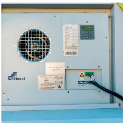
500kW/1075kWh Integrated Energy Storage System...
